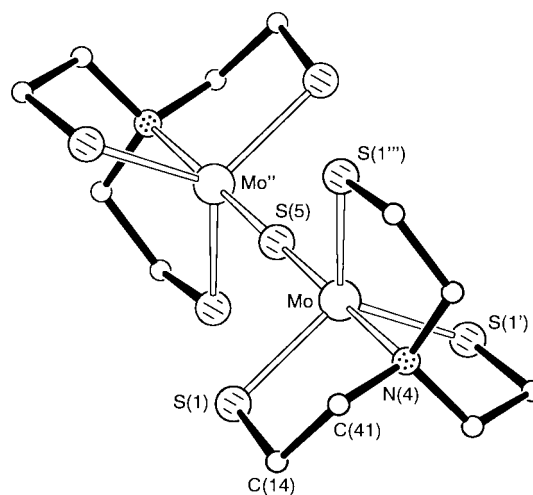
Fig. 1 A molecule of \{[Mo(NS_3)_2(\mu-S)]\} in crystals of 2 . A threefold symmetry axis passes through the length of the molecule and the bridging sulfur atom S(5) lies on a centre of symmetry. For clarity, hydrogen atoms have been omitted in all the figures.
